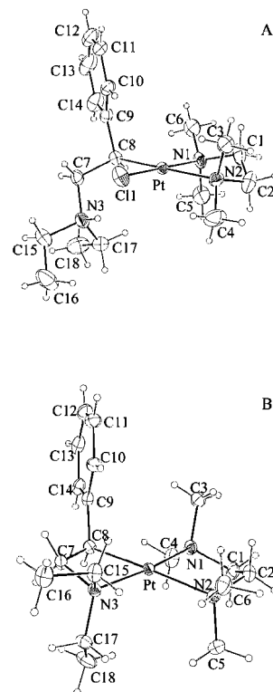
Figure 1. (A) ORTEP drawing of the complex cation [PtCl\{CH(Ph)CH_2NHtEt_2\}(tmeda)]^+ ; the ellipsoids enclose 20% probability. (B) ORTEP drawing of the complex cation [Pt\{CH(Ph)CH_2NET_2-\kappa C,\kappa N\}(tmeda)]^+ ; the ellipsoids enclose 20% probability.
